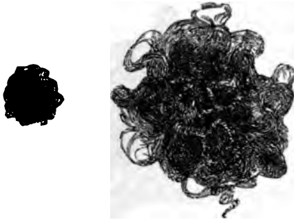
FIG. 109.—COLONIES IN A PLATE-CULTIVATION, \times 70 .
